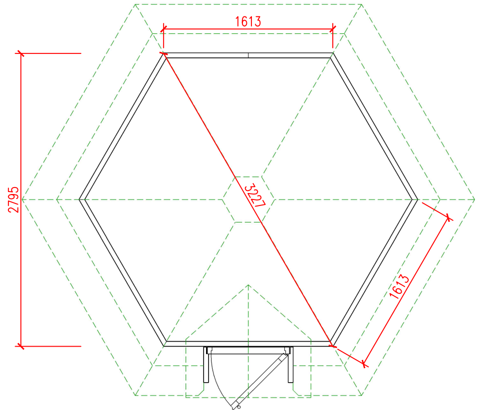
Foundation plan
